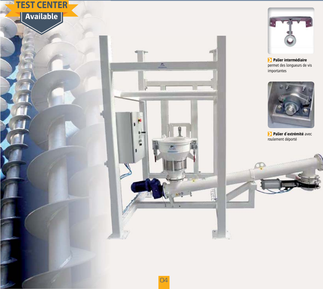
▶ Fond à multi-sorties
